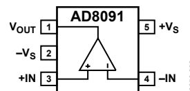
Figure 2. SOT23-5 (RJ-5)
