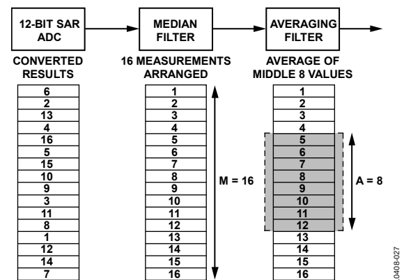
Figure 27. Median and Averaging Filter Example
