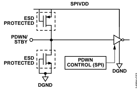
Figure 54. PDWN/STBY Input
