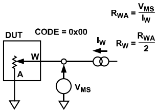
Figure 40. Wiper Resistance
