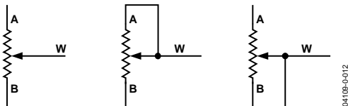
Figure 37. Rheostat Mode Configuration
