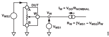
Figure 28. Test Circuit for Wiper Resistance
