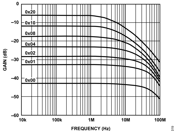
Figure 19. 5 k Ohm Gain vs. Frequency vs. Code
