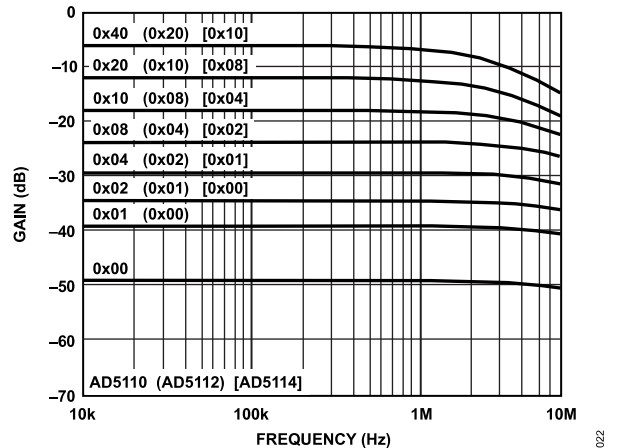
Figure 22. 10 k Ohm Gain vs. Frequency vs. Code
