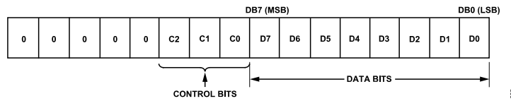
Figure 2. Input Register Content
