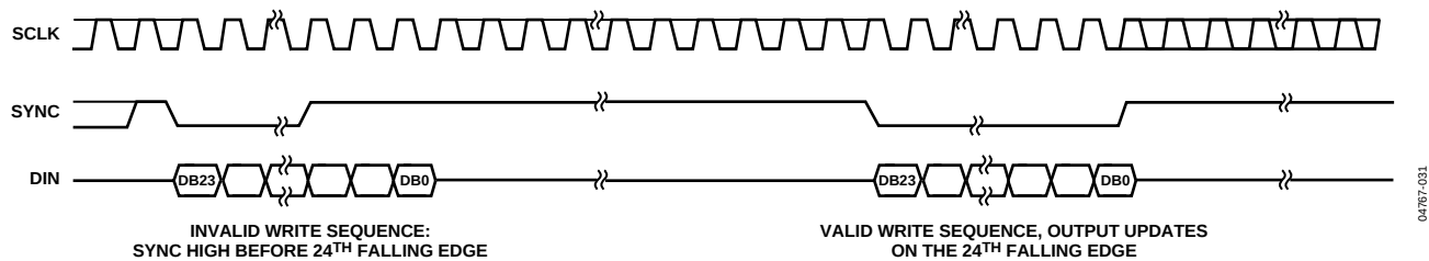
Figure 43. AD5060 \overline{\text{SYNC}} Interrupt Facility
