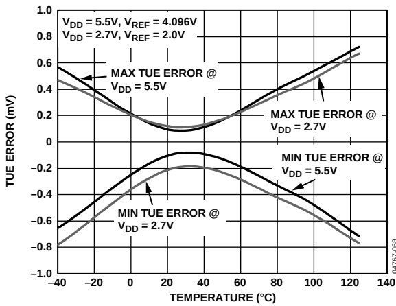
Figure 17. Typical TUE Error vs. Temperature 1
