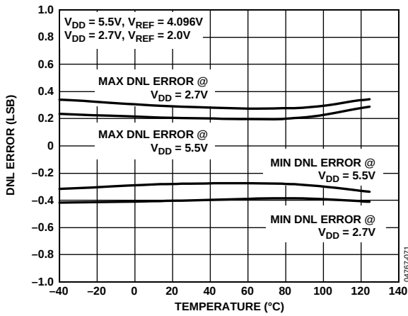
Figure 16. Typical DNL Error vs. Temperature 1
