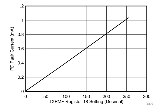
Figure 19. Photodiode Current Monitor Fault vs TXPMF Register Setting
