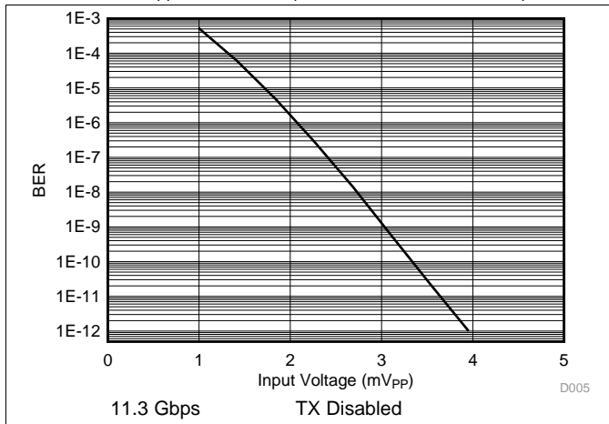
Figure 26. RX Bit-Error Ratio vs Input Amplitude
