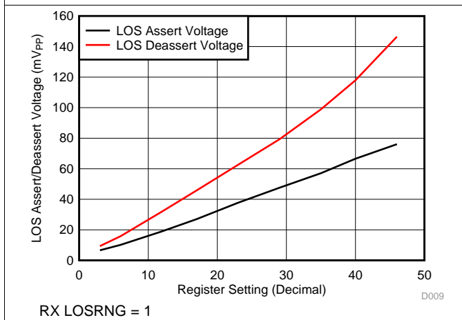
Figure 30. LOS Assert / Deassert Voltage vs Register 7 Setting
