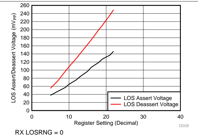
Figure 29. LOS Assert / Deassert Voltage vs Register 7 Setting
