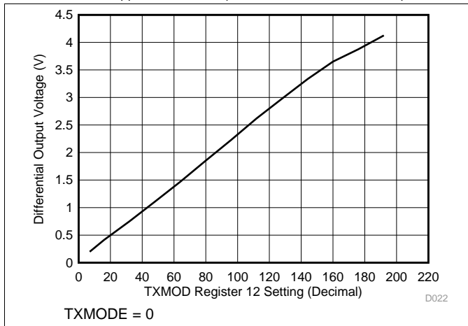
Figure 14. Output Voltage vs Modulation Current
