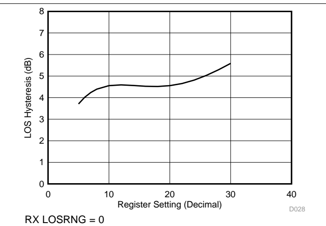
Figure 31. LOS Hysteresis vs Register 7 Setting
