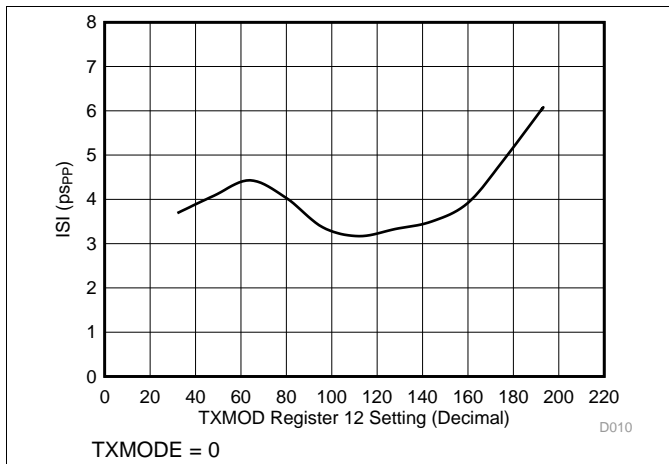
Figure 2. TX Deterministic Jitter vs Modulation Current
