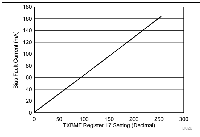
Figure 18. Bias Current Monitor Fault vs TXBMF Register Setting
