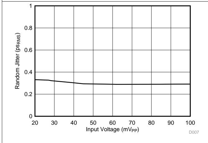
Figure 28. RX Random Jitter vs Input Amplitude
