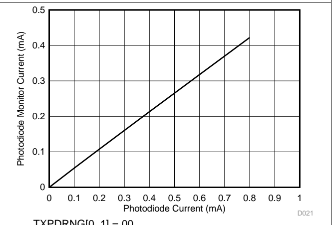
Figure 13. Photodiode-Monitor Current I_{(MONP)} vs PD Current
