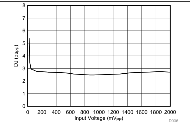
Figure 27. RX Deterministic Jitter vs Input Amplitude
