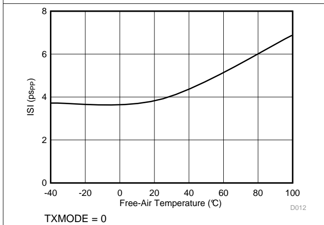
Figure 4. TX Deterministic Jitter vs Temperature
