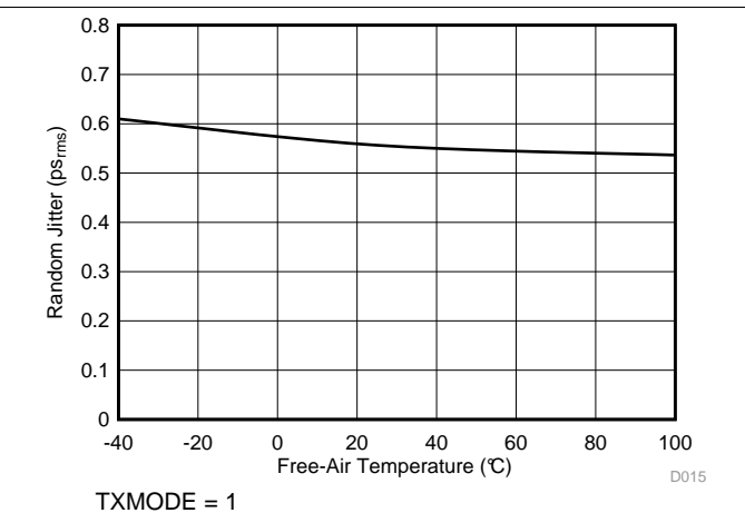
Figure 7. TX Random Jitter vs Temperature
