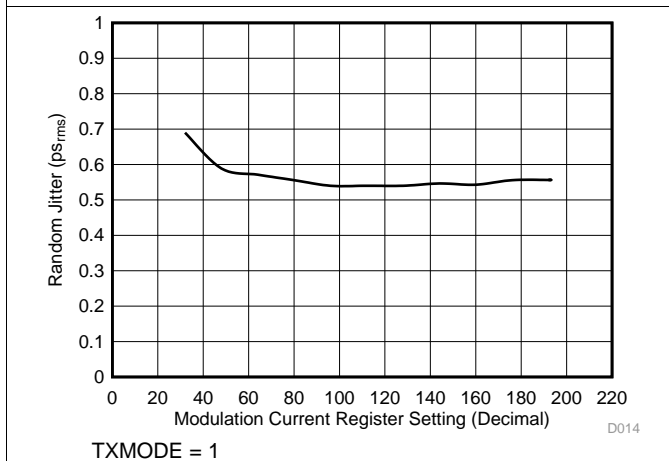
Figure 6. TX Random Jitter vs Modulation Current
