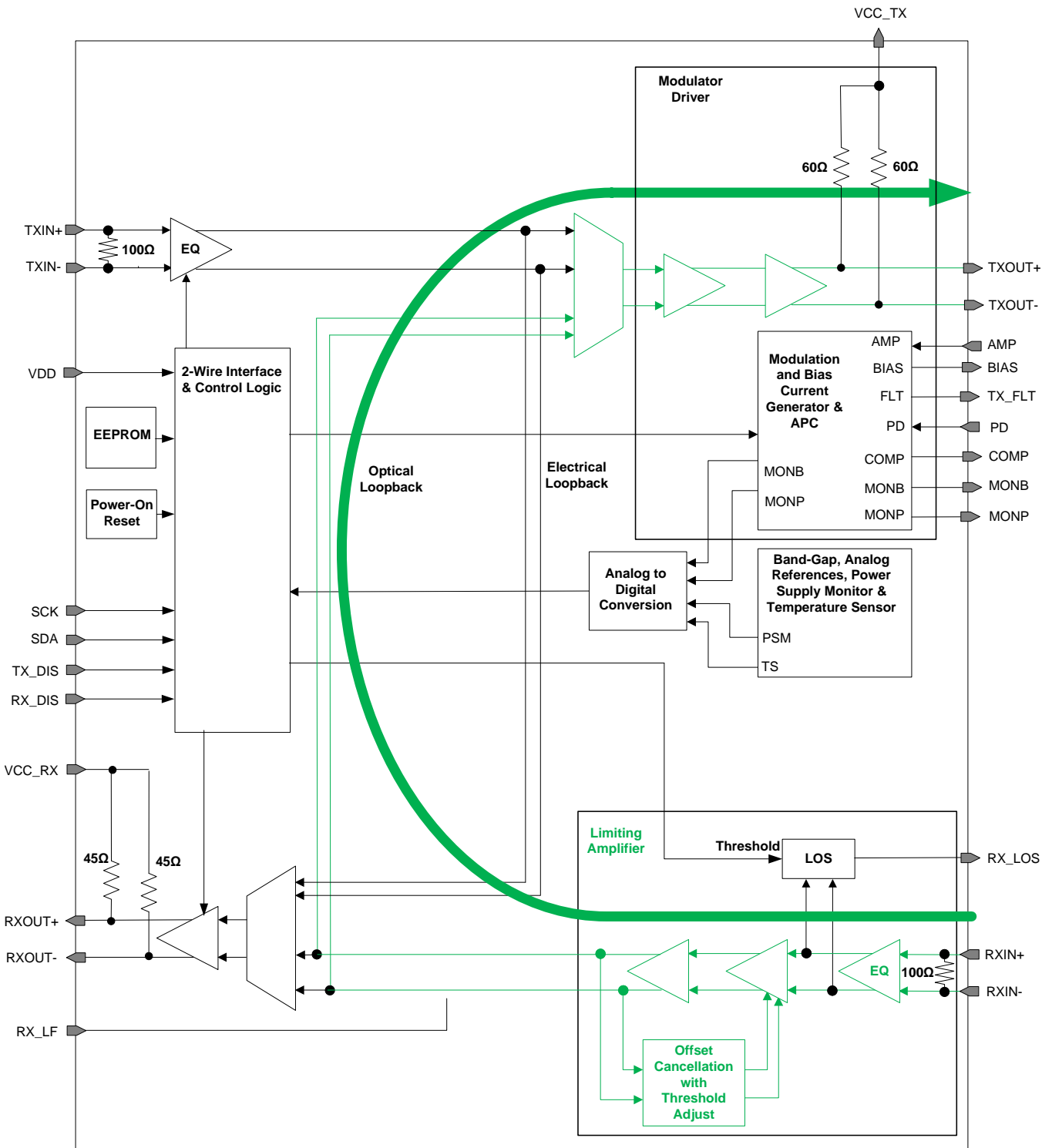
Figure 36. Optical Loopback
