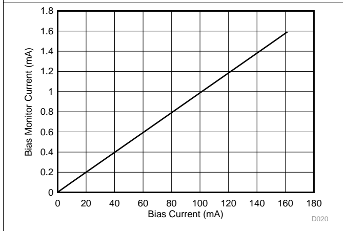
Figure 12. Bias-Monitor Current I_{(MONB)} vs Bias Current
