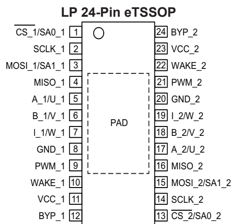
Pinout Diagram
