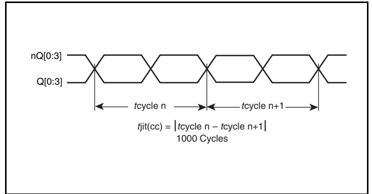
Cycle-to-Cycle Jitter
