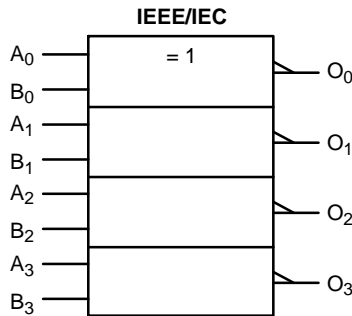
Figure 1. Logic Symbol
