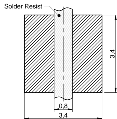
No vias and traces in restricted area. Scale - 10:1
