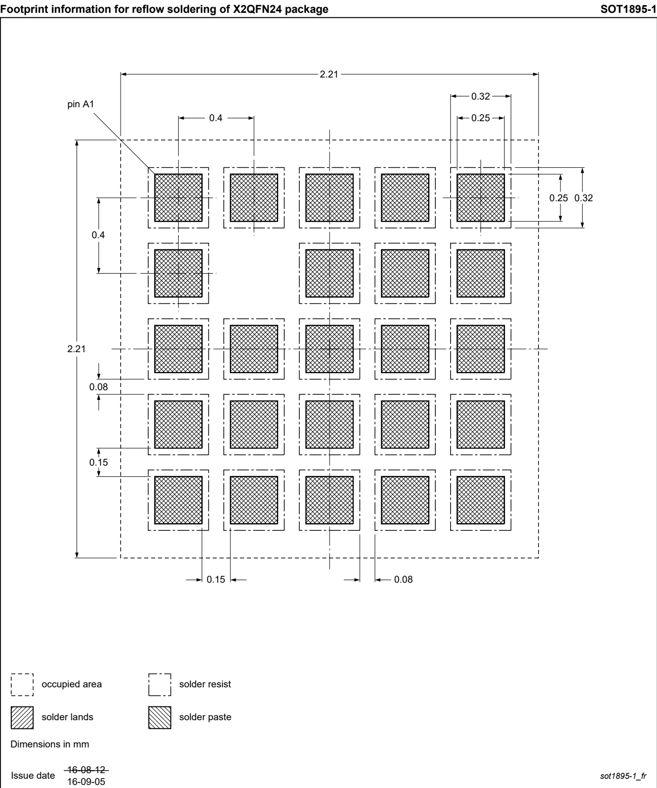
Figure 47. PCB footprint for SOT1895-1 (X2QFN24); reflow soldering
