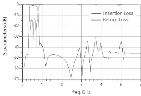
RFBPF3225180C07B1U
