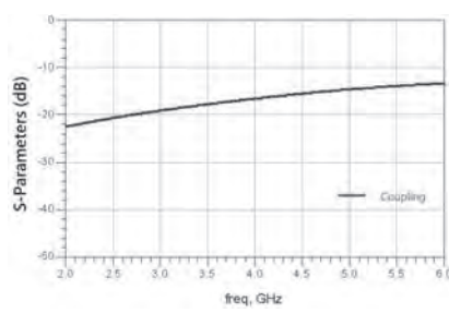
RFCPL0605030L6T
