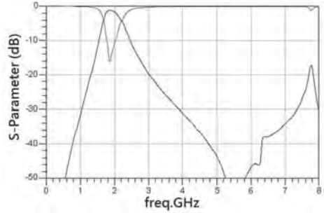
RFBPF1109B501T
