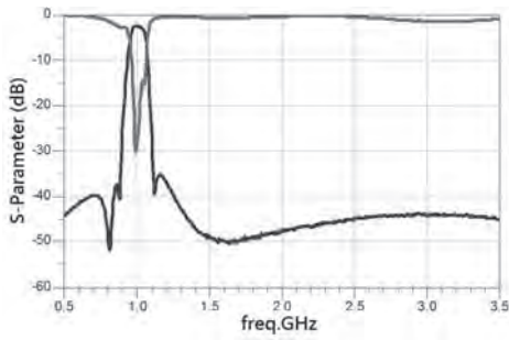
RBBPF3225180Y27B1U
