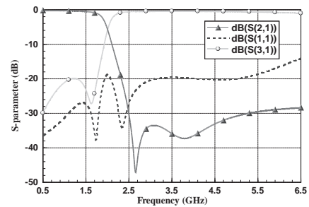
RFDIP1608060TCT
