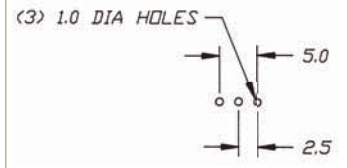
P.C. MOUNTING
