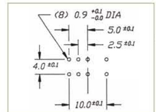
P.C. MOUNTING
