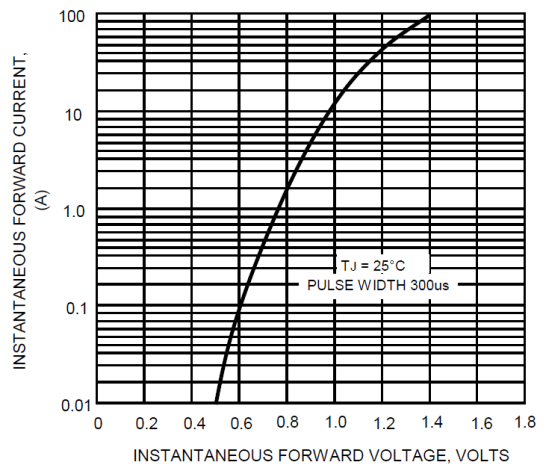
FIG.4-TYPICAL FORWARD CHARACTERISTICS
