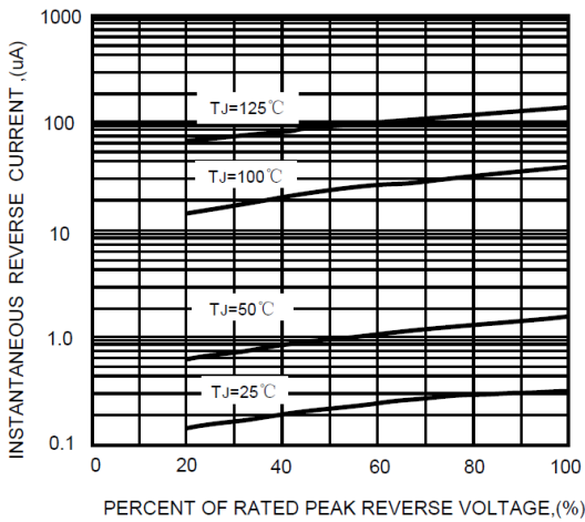
FIG.3-TYPICAL REVERSE CHARACTERISTICS
