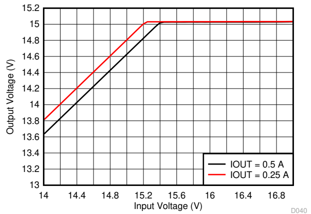
Figure 7-4. Dropout Voltage
