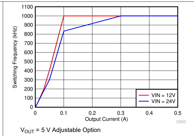
Figure 7-26. Auto PFM Mode Switching Frequency vs Output Current
