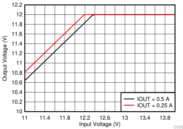
Figure 7-3. Dropout Voltage
