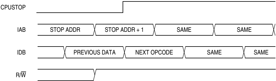
Figure 9-17. Stop Mode Entry Timing
