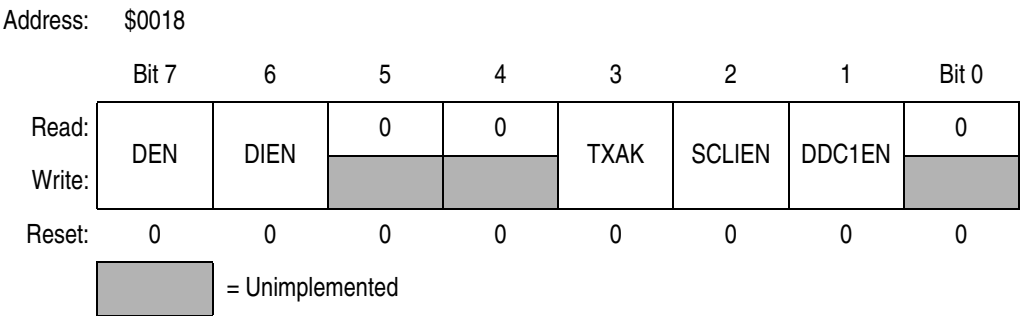
Figure 16-4. DDC Control Register (DDCCR)
