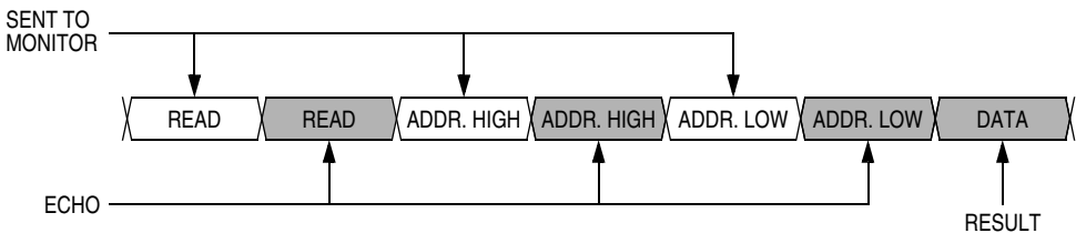
Figure 10-4. Read Transaction
