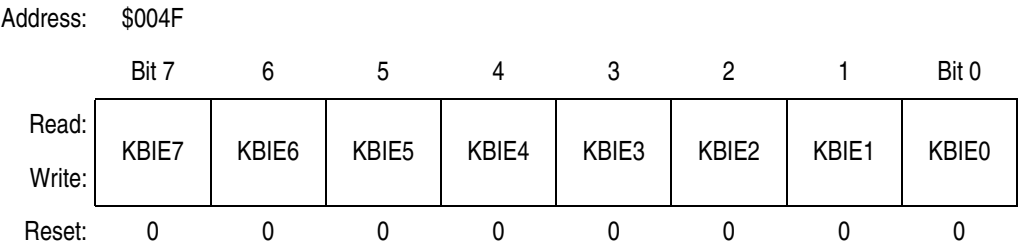
Figure 19-5. Keyboard Interrupt Enable Register (KIER)
