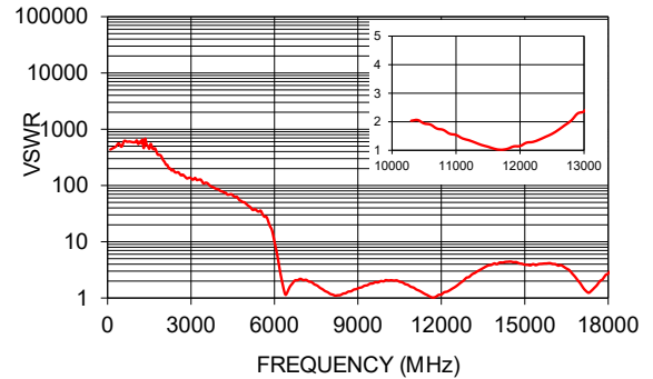
HFCN-672+ VSWR
