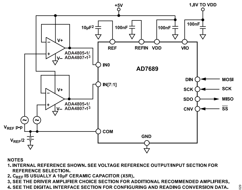
Figure 29. Typical Application Diagram Using Bipolar Input
