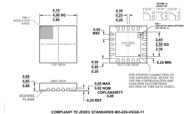
Figure 47. 20-Lead Lead Frame Chip Scale Package [LFCSP] 4 mm × 4 mm Body and 0.85 mm Package Height (CP-20-22) Dimensions shown in millimeters
