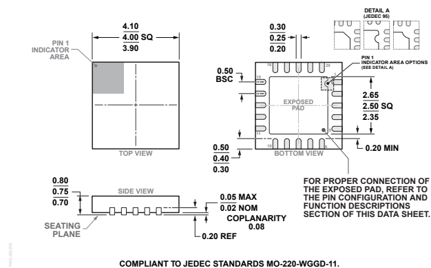
Figure 46. 20-Lead Lead Frame Chip Scale Package [LFCSP] 4 mm × 4 mm Body and 0.75 mm Package Height (CP-20-10) Dimensions shown in millimeters
