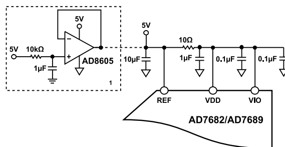
Figure 38. Example of an Application Circuit
