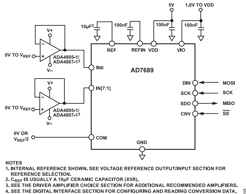
Figure 28. Typical Application Diagram with Multiple Supplies
