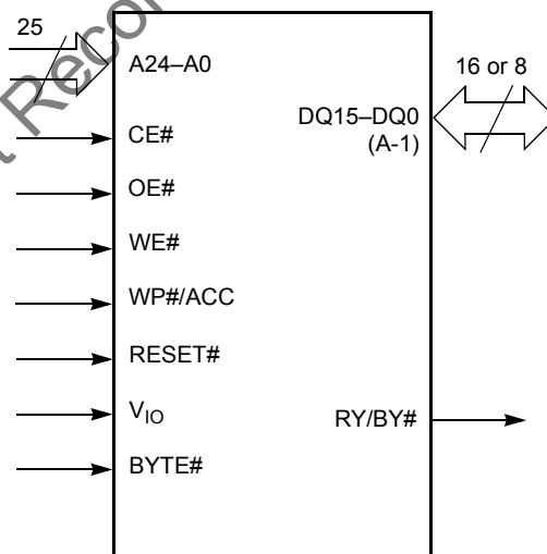
Figure 5.1 S29GL512N
