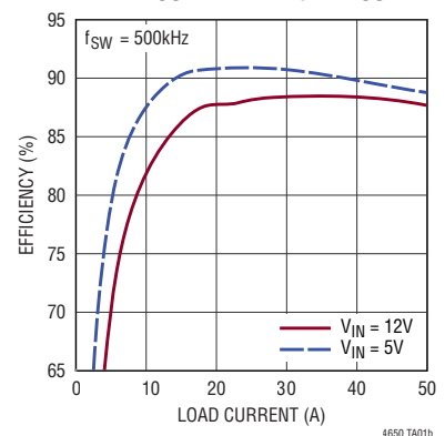
1.2V OUT Efficiency vs I OUT
