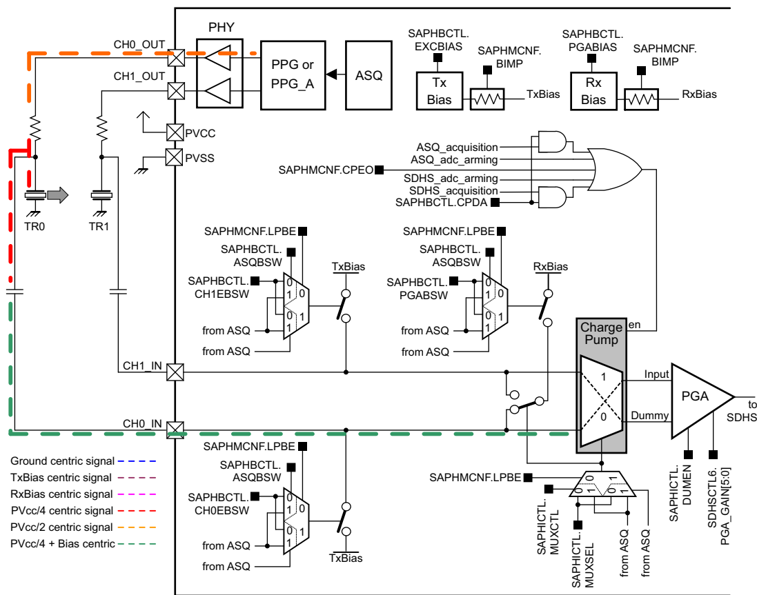
Figure 21-15. Excitation
