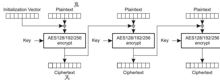
Figure 14-8. CBC Encryption
