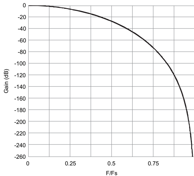
Figure 22-6. SDHS Filter Frequency Response Within f_s , SDHSCTL1.OSR = 10
