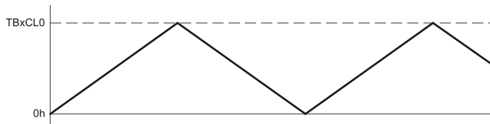
Figure 26-7. Up/Down Mode
