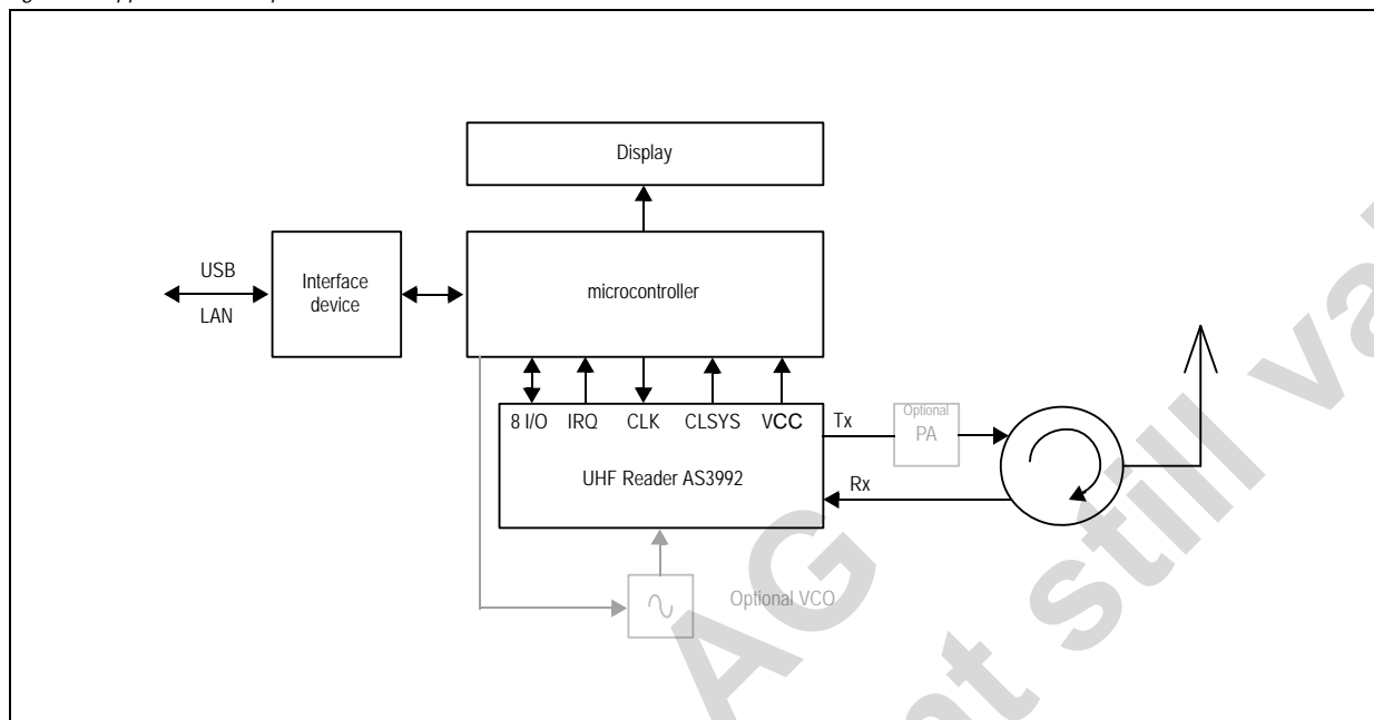
Figure 5. Application Example
