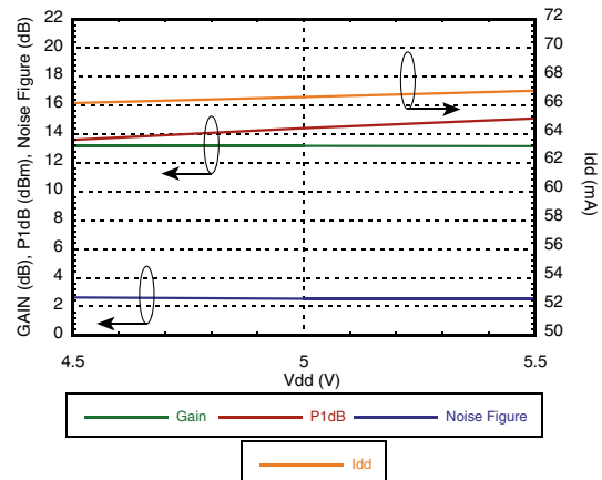
Gain, Power, Noise Figure & Supply Current vs. Supply Voltage @ 10 GHz
