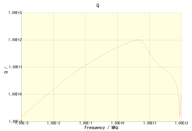
CLF12555T-2R2N-CA
