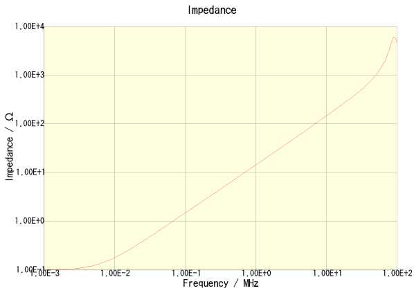
CLF12555T-2R2N-CA
