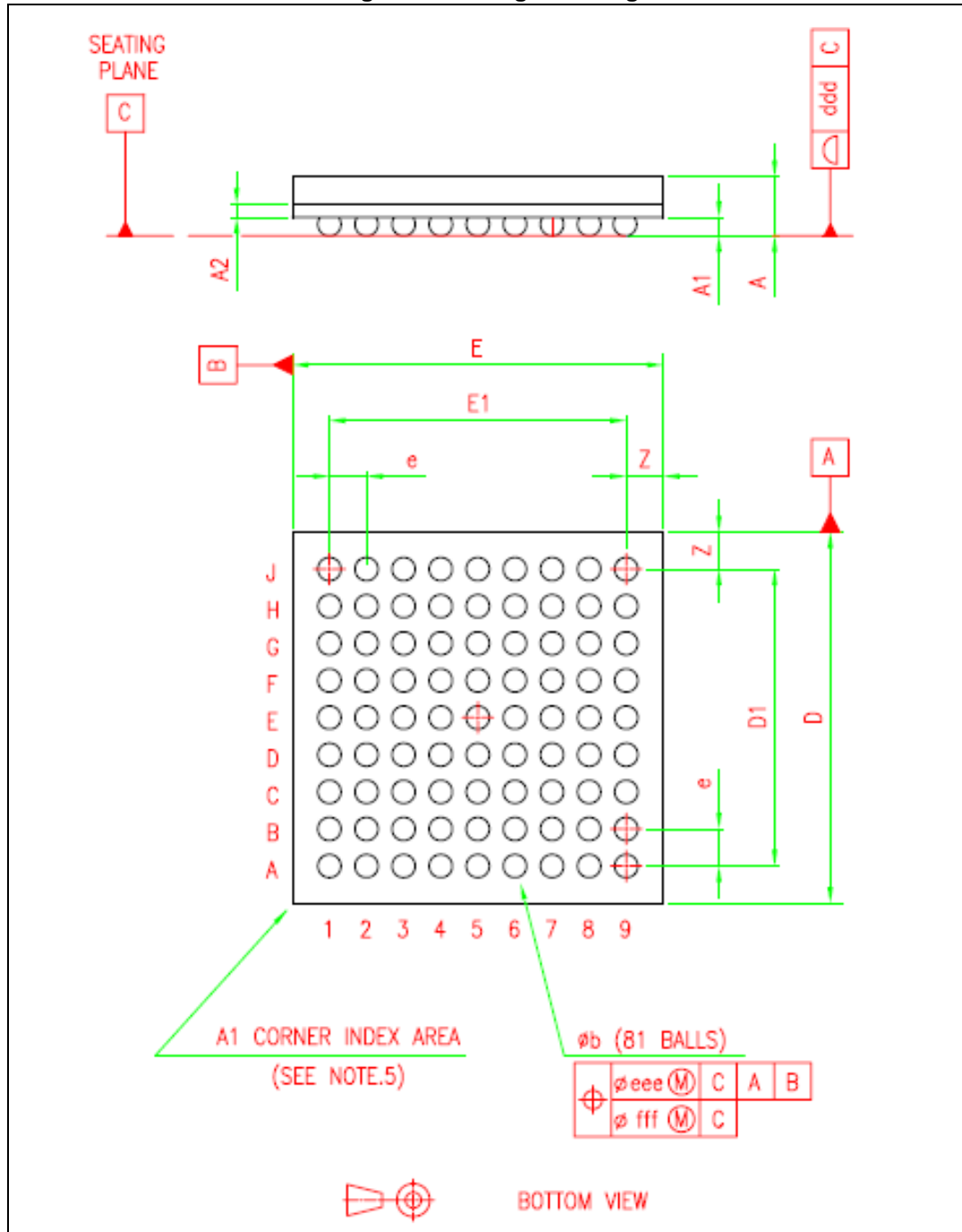
Figure 4. Package drawing
