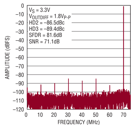
LTC6409 Driving LTC2262-14 ADC, f_{\text{IN}} = 70\text{MHz} , -1dBFS, f_{\text{s}} = 150\text{MHz} , 4096-Point FFT
