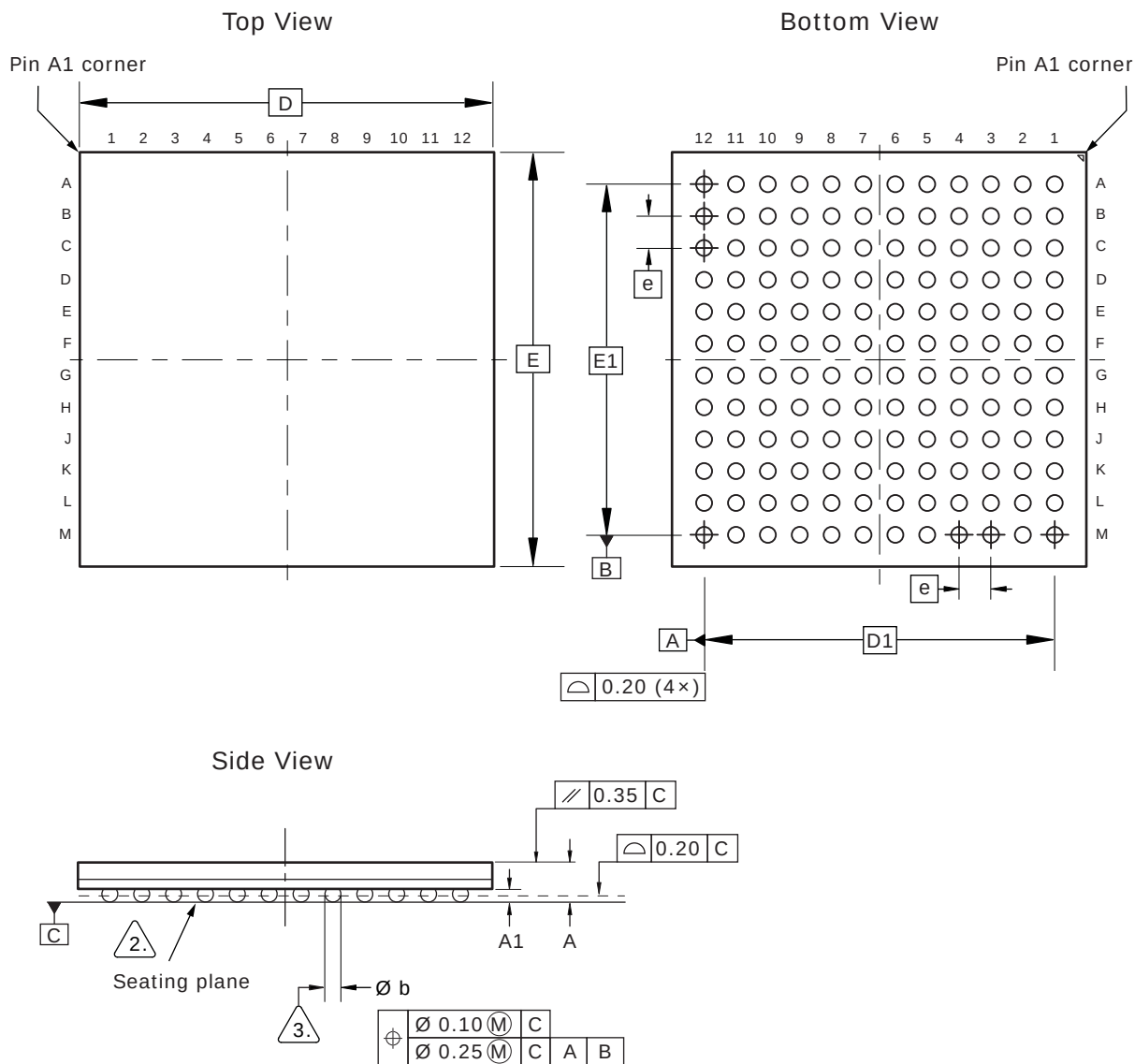
Figure 64 • Package Drawing
