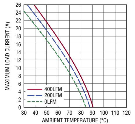
Figure 22. 24V to 1.8V Derating Curve, No Heat Sink
