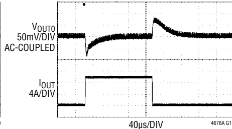
FIGURE 69 CIRCUIT AT 24V_{IN} . C OUT0 = 5 \times 100\mu\text{F} AND VOUT0 COMMANDED TO 3.300V. 0A TO 10A LOAD STEP AT 10A/\mu\text{s}
