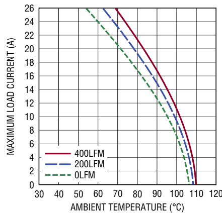
Figure 18. 12V to 1V Derating Curve, with Heat Sink
