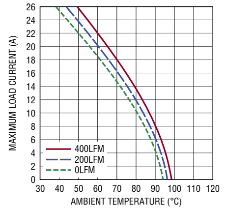
Figure 16. 24V to 1V Derating Curve, No Heat Sink
