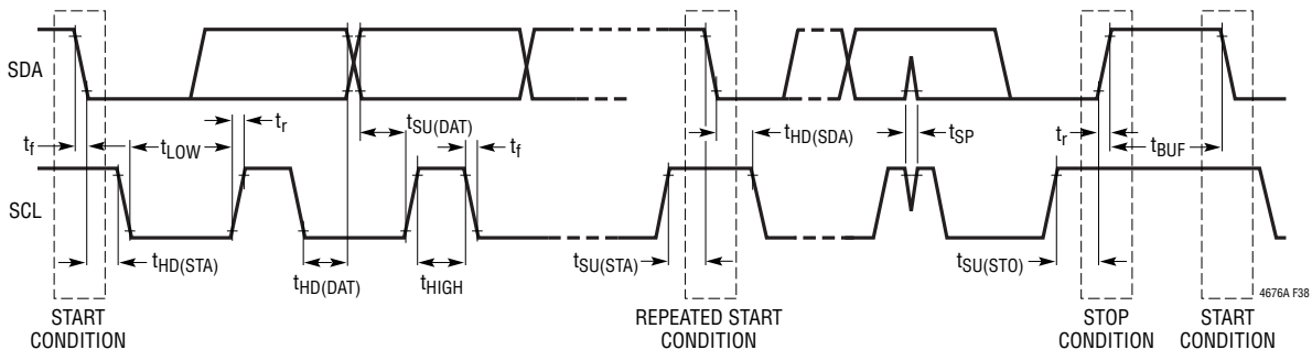
Figure 44. Timing Diagram
