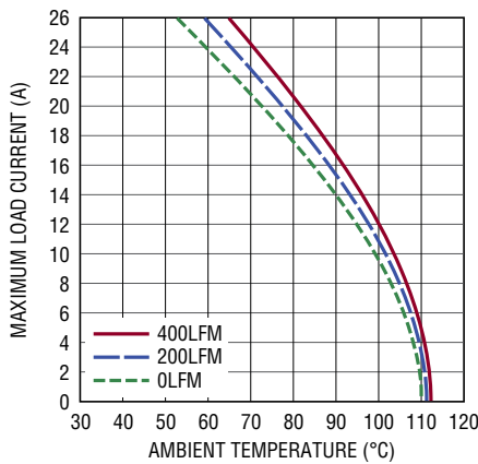
Figure 20. 5V to 1.8V Derating Curve, No Heat Sink
