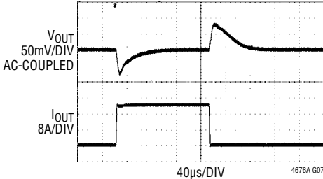
FIGURE 35 CIRCUIT AT 12V_{IN} . INTV CC PIN OPEN CIRCUIT AND VOUT_COMMAND n SET TO 1.000V. 0A TO 20A LOAD STEP AT 20A/\mu\text{s}
