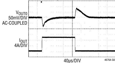
FIGURE 69 CIRCUIT AT 12V_{IN} . 0A TO 10A LOAD STEP AT 10A/\mu\text{s}
