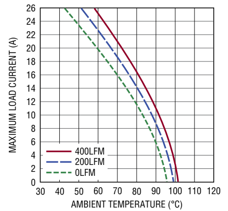
Figure 19. 24V to 1V Derating Curve, with Heat Sink
