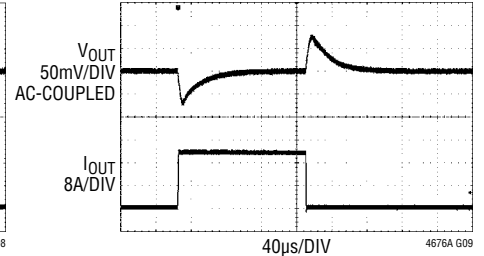
FIGURE 35 CIRCUIT AT 5V_{IN} . VOUT_COMMAND n SET TO 1.000V. 0A TO 20A LOAD STEP AT 20A/\mu\text{s}
