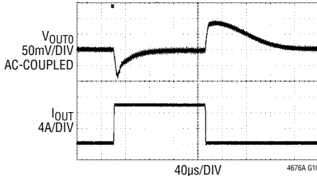
FIGURE 69 CIRCUIT AT 24V_{IN} . 0A TO 10A LOAD STEP AT 10A/\mu\text{s}
