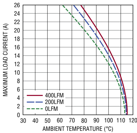
Figure 17. 5V to 1V Derating Curve, with Heat Sink
