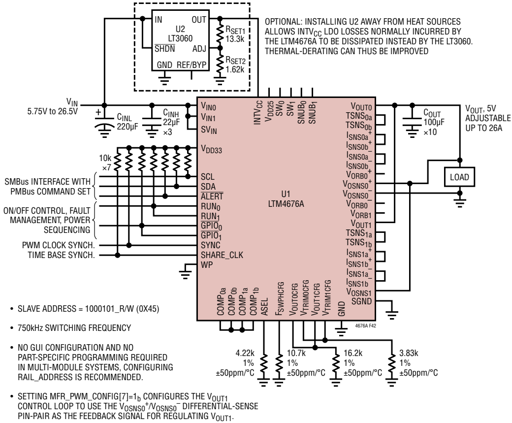
Figure 42. 26A, 5V Output DC/DC \mu Module Regulator with Serial Interface
