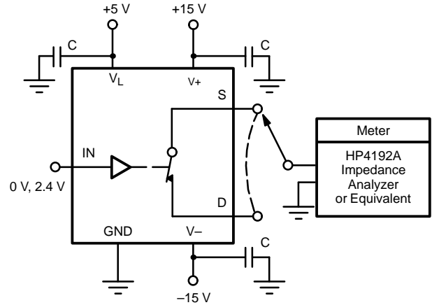
FIGURE 7. Source/Drain Capacitances
