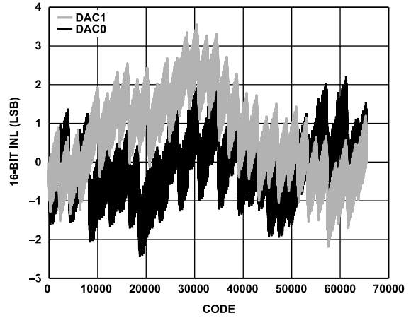
Figure 36. INL, I_{OUTFS} = 15.6\text{ mA} , 16-Bit Resolution
