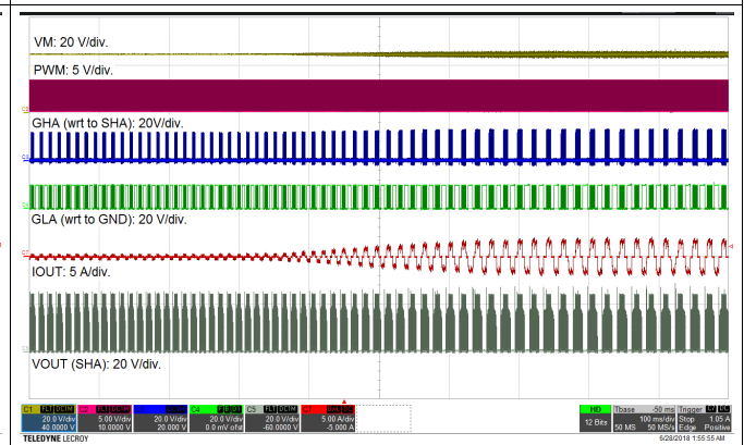
Figure 42. Motor Performance at Load Change
