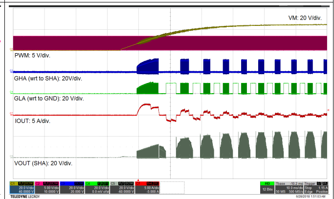
Figure 40. Motor Starting With Supply Voltage Change
