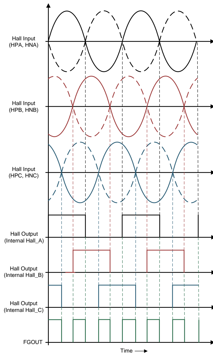
Figure 21. FGOUT Signal
