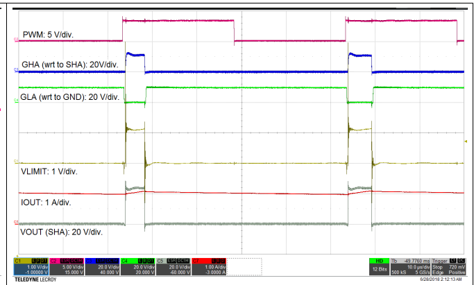
Figure 38. VLIMIT Operation
