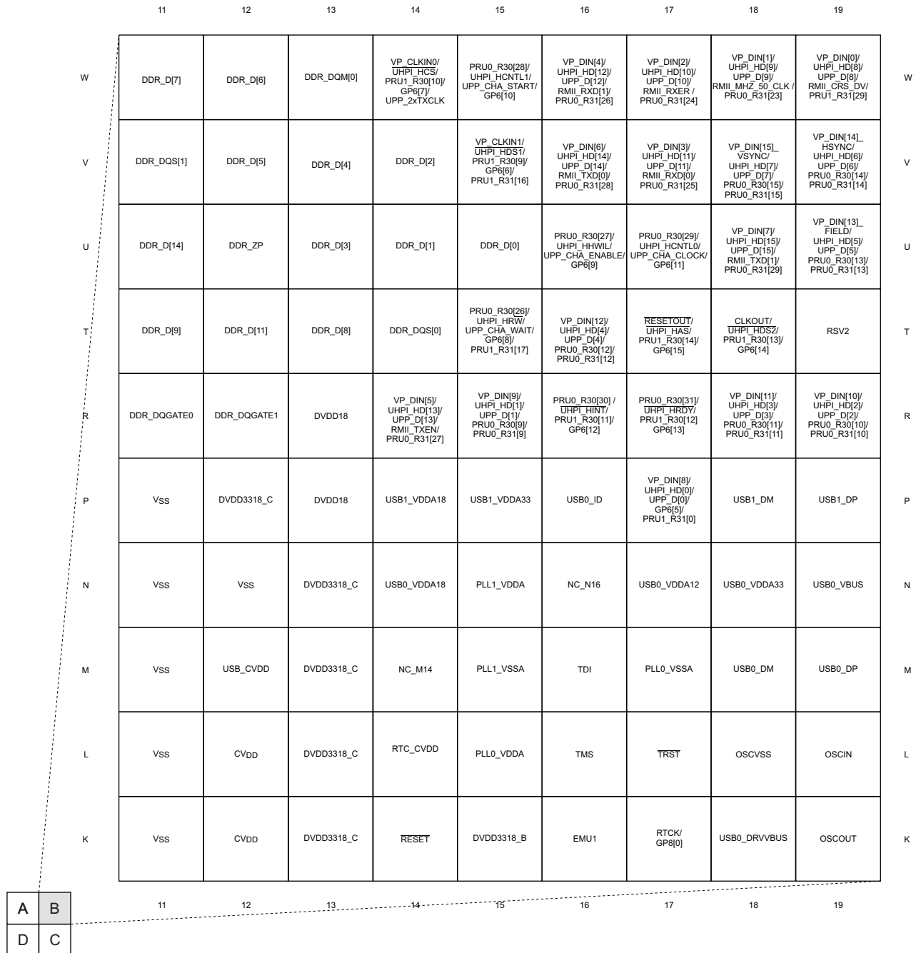
Figure 2-2. Pin Map (Quad B)
