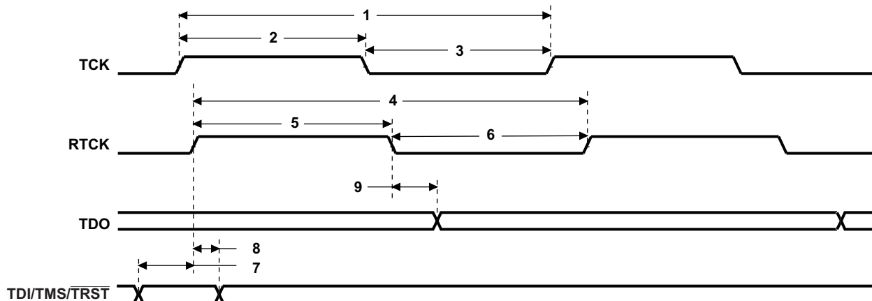
Figure 5-89. JTAG Test-Port Timing
