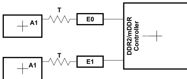
Figure 5-22. DQS and D Routing and Topology
