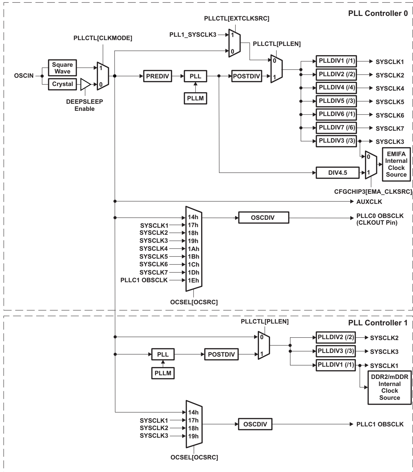
Figure 5-9. PLL Topology
