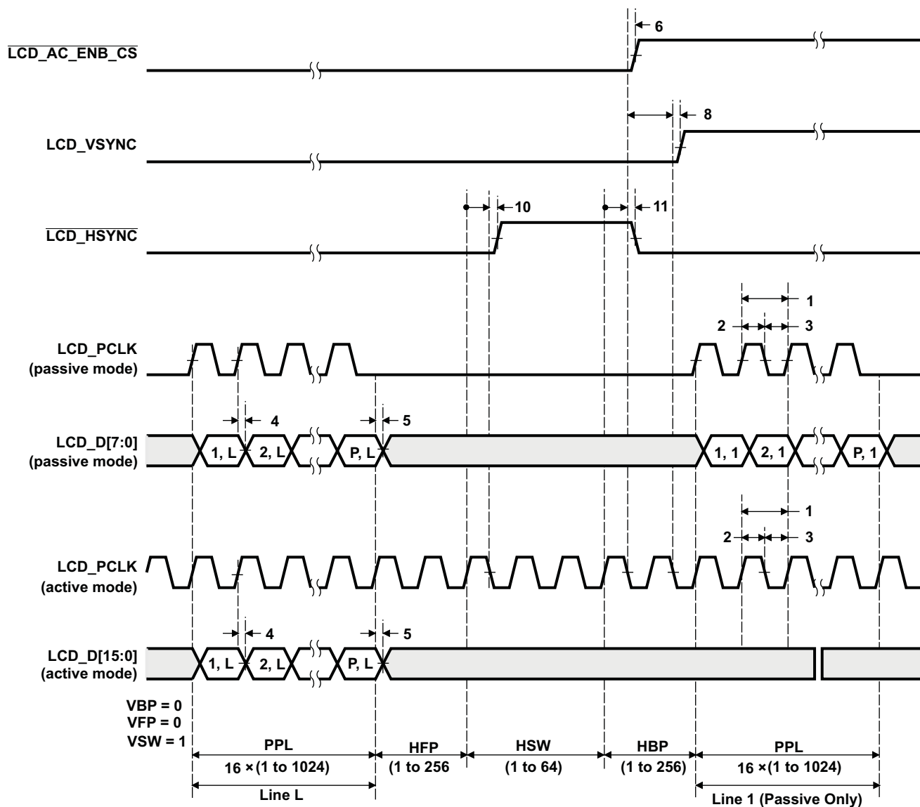
Figure 5-63. LCD Raster-Mode Control Signal Activation
