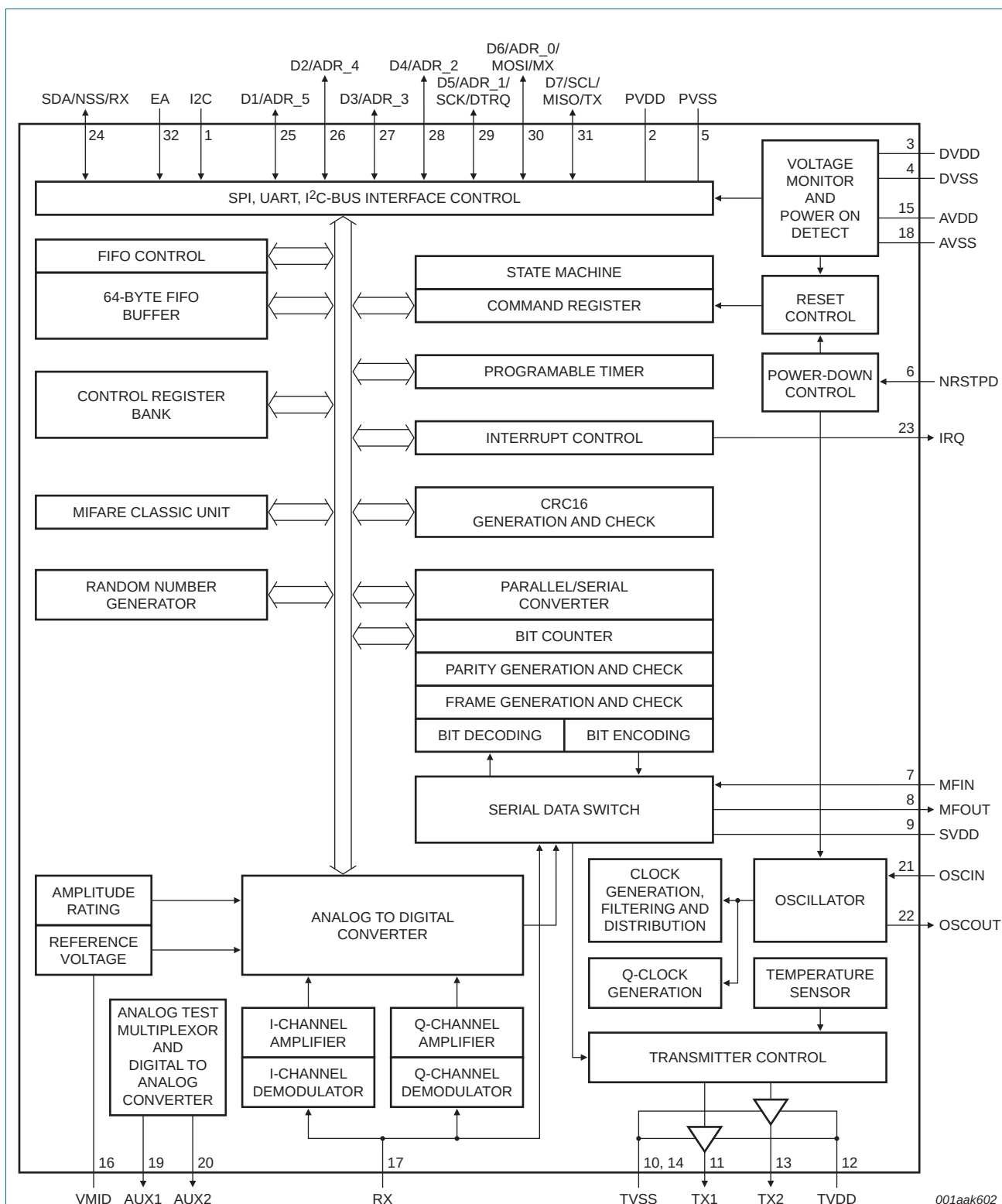
Fig 2. Detailed block diagram of the MFRC522
