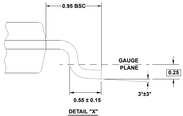
DETAIL "X"
