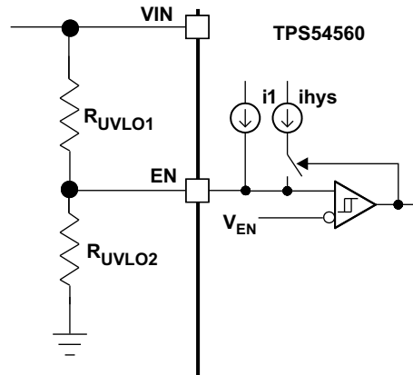
Figure 22. Adjustable Undervoltage Lockout (UVLO)
