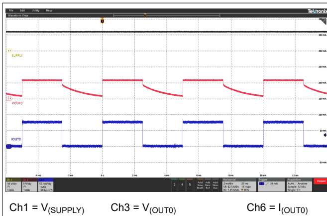
Figure 6-11. PWM Dimming at 200 Hz
