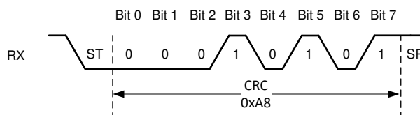
Figure 7-15. CRC Byte
