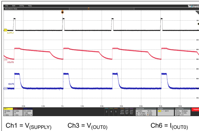
Figure 6-13. Supply Dimming In Fail-Safe Mode
