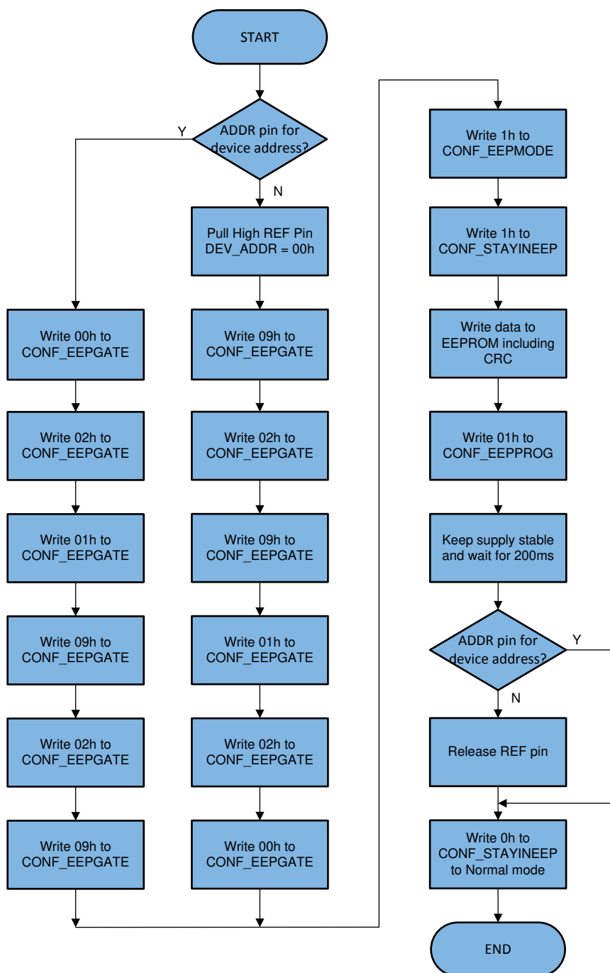
Figure 7-18. Programming Sequence
