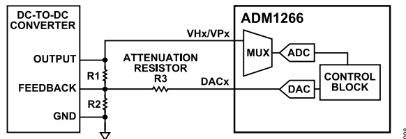
Figure 12. Typical Application Circuit for Margining
