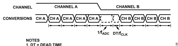
Figure 99. Fast Settling, \text{Sinc}^4 + \text{Sinc}^1 Filter
