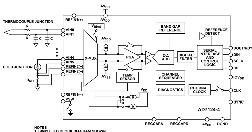
Figure 127. Thermocouple Application
