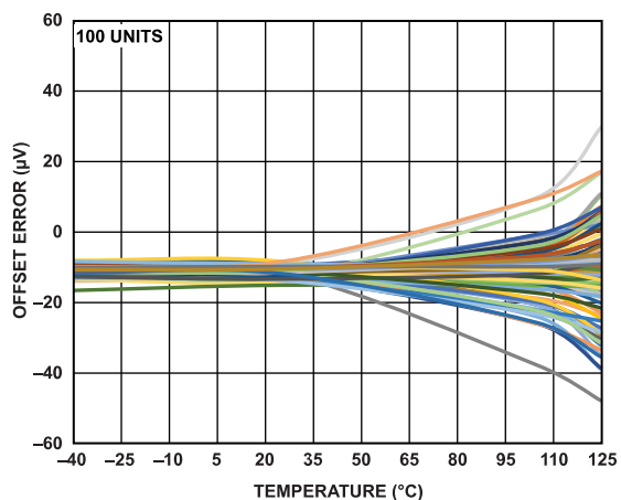
Figure 19. Input Referred Offset Error vs. Temperature (Gain = 8, Low Power Mode)
