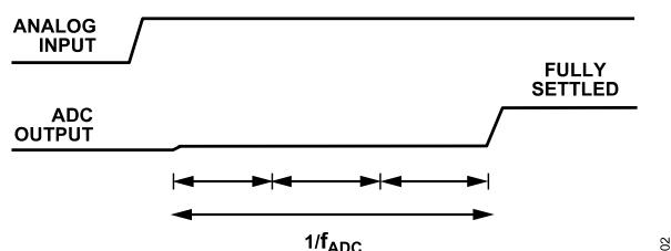
Figure 93. Sinc 3 Zero Latency Operation
