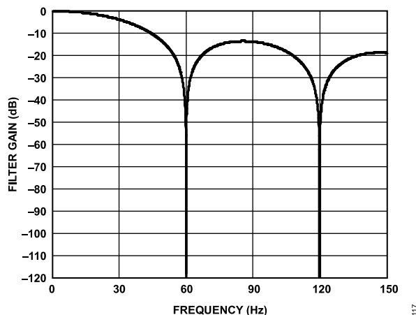
Figure 108. 60 Hz Rejection
