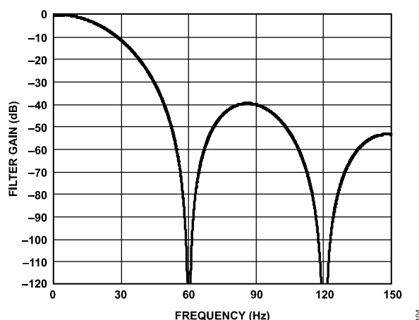
Figure 95. Sinc 3 Filter Response (60 SPS Output Data Rate, Zero Latency Disabled or 20 SPS Output Data Rate, Zero Latency Enabled)
