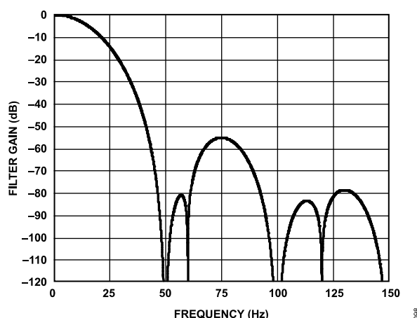
Figure 89. \text{sinc}^4 Filter Response (50 SPS Output Data Rate, Zero Latency Disabled or 12.5 SPS Output Data Rate, Zero Latency Enabled, REJ60 = 1)
