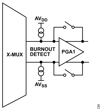
Figure 125. Burnout Currents
