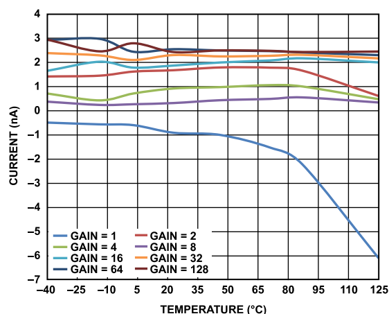
Figure 45. Differential Analog Input Current vs. Temperature (Mid Power Mode)
