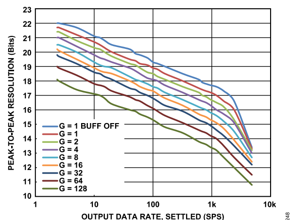
Figure 49. Peak-to-Peak Resolution vs. Output Data Rate (Settled), \text{Sinc}^4 Filter (Full Power Mode)
