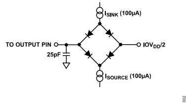
Figure 2. Load Circuit for Timing Characterization
