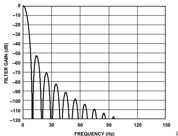
Figure 88. \text{sinc}^4 Filter Response (10 SPS Output Data Rate, Zero Latency Disabled or 2.5 SPS Output Data Rate, Zero Latency Enabled)
