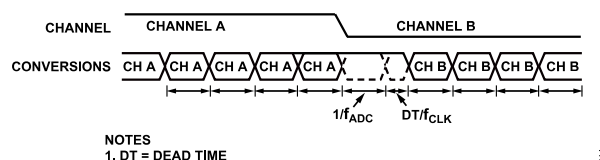
Figure 105. Fast Settling, \text{Sinc}^3 + \text{Sinc}^1 Filter
