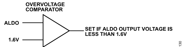
Figure 121. Analog LDO Monitor
