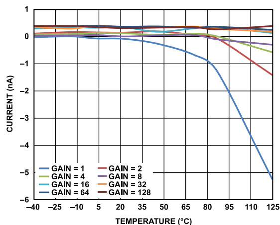
Figure 46. Differential Analog Input Current vs. Temperature (Low Power Mode)
