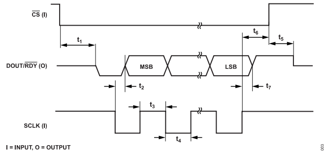
Figure 3. Read Cycle Timing Diagram ( \overline{\text{CS}}_{\text{EN}} Bit Cleared)
