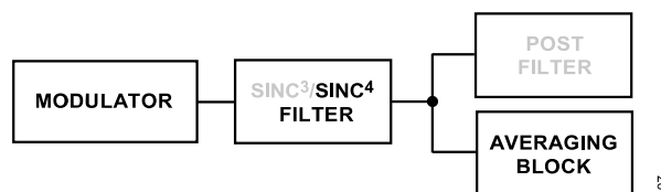
Figure 98. Fast Settling Mode, Sinc 4 + Sinc 1 Filter
