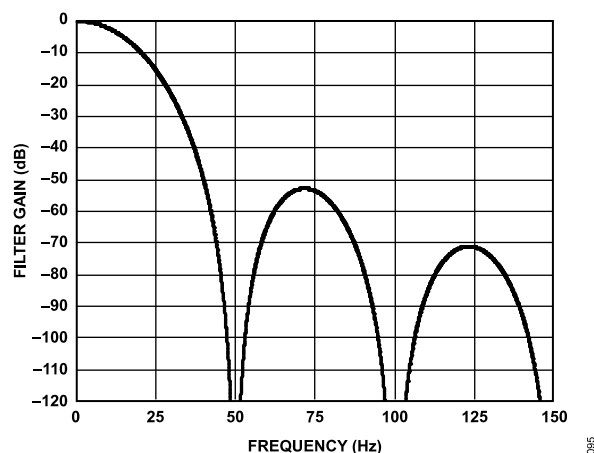
Figure 86. \text{sinc}^4 Filter Response (50 SPS Output Data Rate, Zero Latency Disabled or 12.5 SPS Output Data Rate, Zero Latency Enabled)
