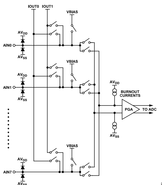
Figure 78. Excitation Current and Bias Voltage Connections
