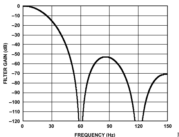
Figure 87. \text{sinc}^4 Filter Response (60 SPS Output Data Rate, Zero Latency Disabled or 15 SPS Output Data Rate, Zero Latency Enabled)
