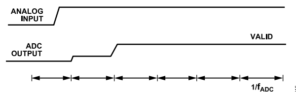
Figure 106. Step Change on the Analog Input, \text{Sinc}^3 + \text{Sinc}^1 Filter
