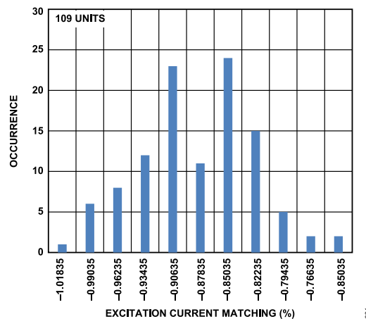
Figure 32. IOUTx Current Initial Matching Histogram (500 µA)
