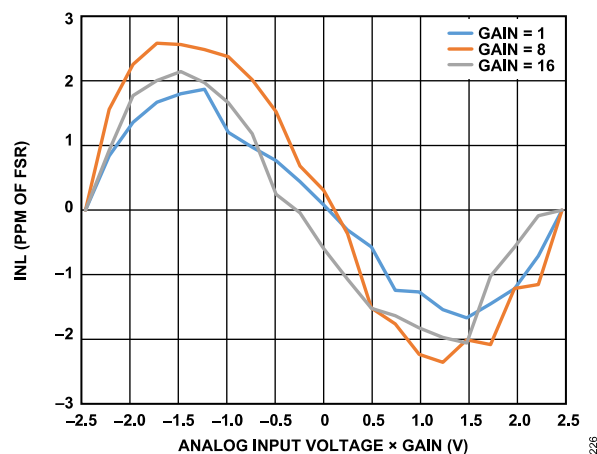
Figure 27. INL vs. Differential Input Signal (Analog Input × Gain), ODR = 50 SPS, External 2.5 V Reference
