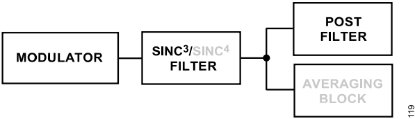
Figure 110. Post Filters
