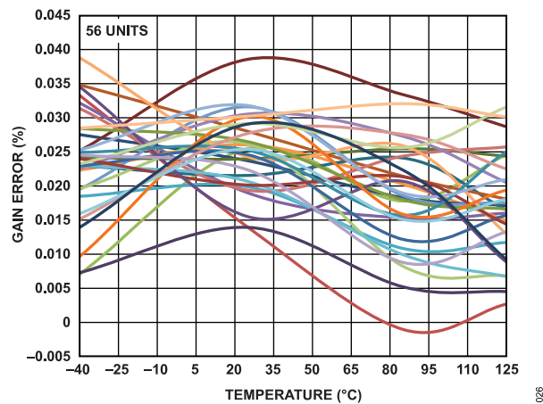
Figure 26. Input Referred Gain Error vs. Temperature (Gain = 16)
