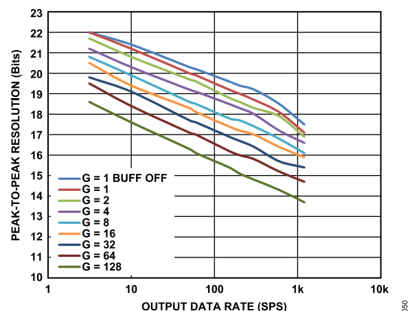
Figure 51. Peak-to-Peak Resolution vs. Output Data Rate, \text{Sinc}^4 + \text{Sinc}^1 Filter (Full Power Mode)
