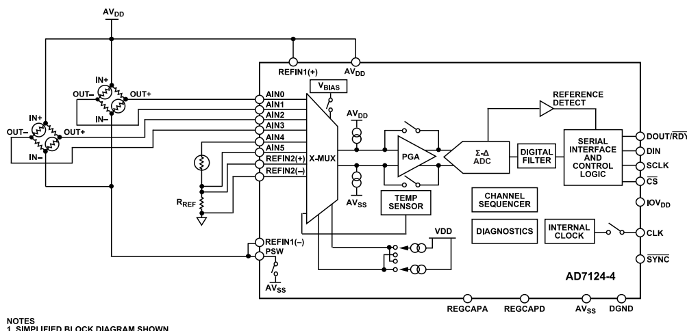
Figure 65. Basic Connection Diagram
