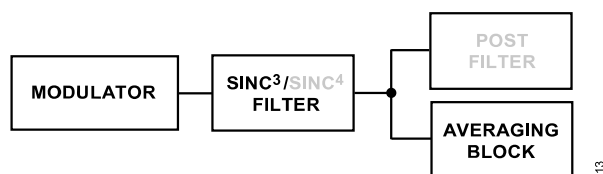
Figure 104. Fast Settling Mode, \text{Sinc}^3 + \text{Sinc}^1 Filter
