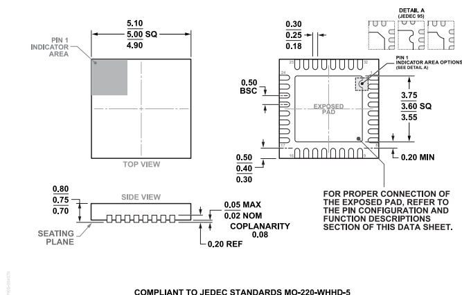
Figure 130. 32-Lead Lead Frame Chip Scale Package [LFCSP] 5 mm × 5 mm Body and 0.75 mm Package Height (CP-32-12) Dimensions shown in millimeters
