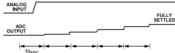
Figure 84. Asynchronous Step Change in the Analog Input
