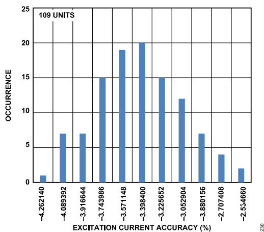
Figure 31. IOUTx Current Initial Accuracy Histogram (500 µA)
