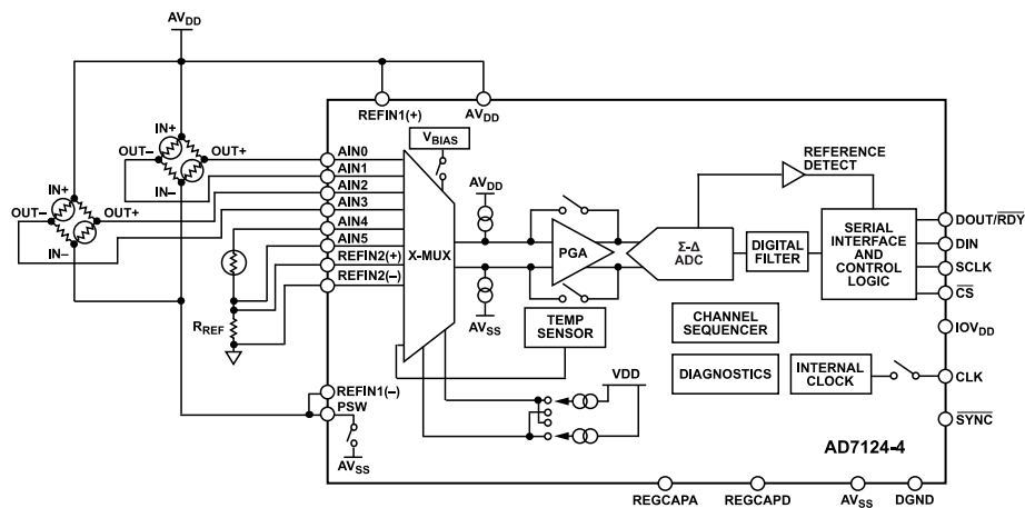
Figure 129. Flowmeter Application
