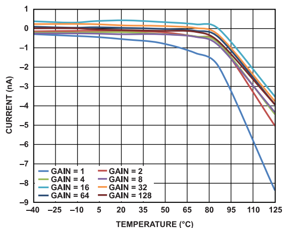
Figure 42. Absolute Analog Input Current vs. Temperature (Mid Power Mode)
