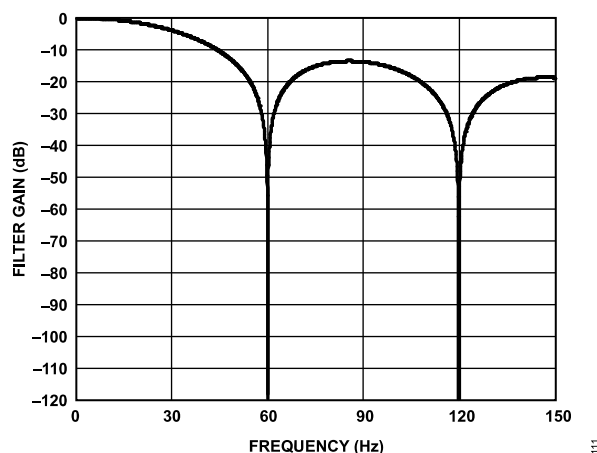
Figure 102. 60 Hz Rejection
