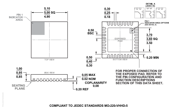
Figure 132. 32-Lead Lead Frame Chip Scale Package [LFCSP] 5 mm × 5 mm Body and 0.95 mm Package Height (CP-32-30) Dimensions shown in millimeters
