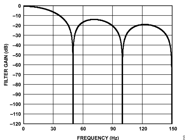
Figure 101. 50 Hz Rejection
