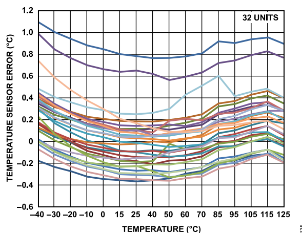
Figure 126. Temperature Sensor Error vs. Temperature
