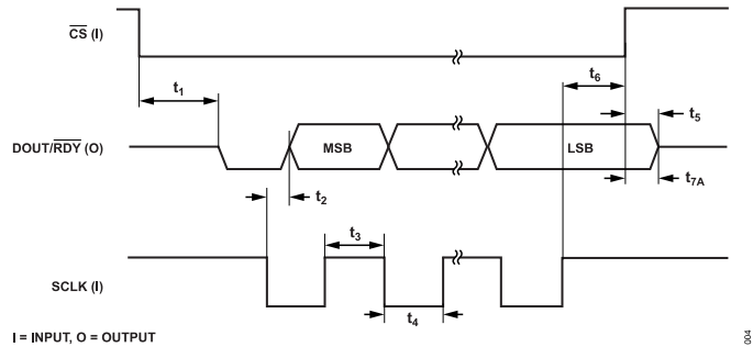
Figure 4. Read Cycle Timing Diagram ( \overline{\text{CS}}_{\text{EN}} Bit Set)
