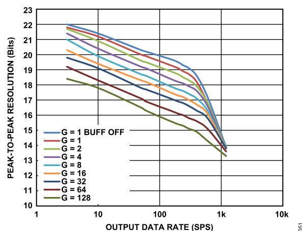
Figure 52. Peak-to-Peak Resolution vs. Output Data Rate, \text{Sinc}^3 + \text{Sinc}^1 Filter (Full Power Mode)
