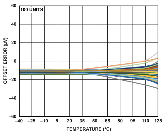
Figure 18. Input Referred Offset Error vs. Temperature (Gain = 8, Mid Power Mode)
