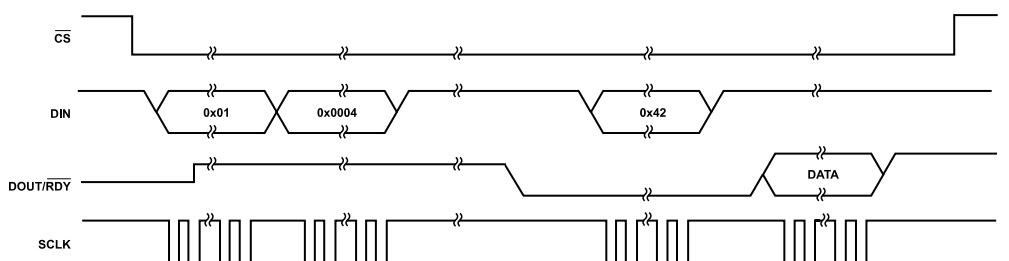
Figure 79. Single Conversion Configuration
