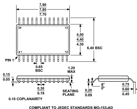
Figure 131. 24-Lead Thin Shrink Small Outline Package [TSSOP] (RU-24) Dimensions shown in millimeters
