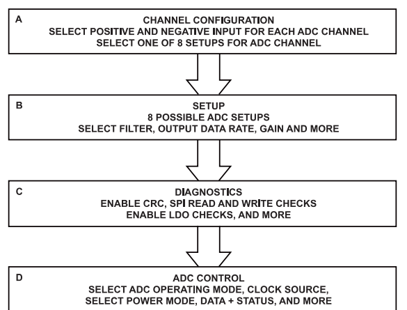
Figure 69. Suggested ADC Configuration Flow
