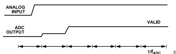
Figure 100. Step Change on the Analog Input, \text{Sinc}^4 + \text{Sinc}^1 Filter
