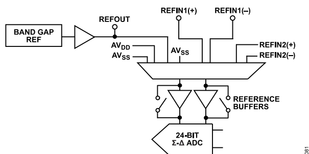
Figure 76. Reference Connections
