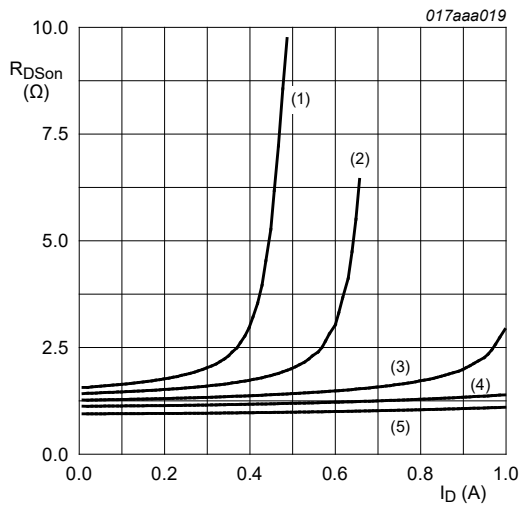
Fig. 8. Drain-source on-state resistance as a function of drain current; typical values (1) V_{GS} = 3.25\text{ V} (2) V_{GS} = 3.5\text{ V} (3) V_{GS} = 4\text{ V} (4) V_{GS} = 5\text{ V} (5) V_{GS} = 10\text{ V}
