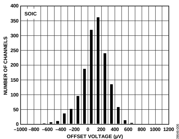
Figure 12. Input Offset Voltage Distribution, V_{SV} = \pm 15\text{ V}
