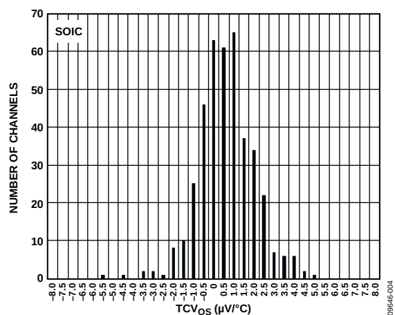
Figure 10. Input Offset Voltage Drift ( TCV_{OS} ) Distribution, V_{SV} = \pm 5\text{ V}
