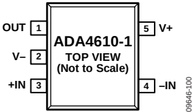
Figure 3. ADA4610-1 Pin Configuration, 5-Lead SOT-23 (RJ Suffix)
