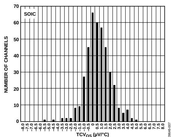
Figure 13. TCV_{OS} Distribution, V_{SV} = \pm 15\text{ V}
