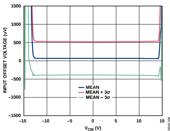
Figure 14. Input Offset Voltage vs. Input Common-Mode Voltage ( V_{CM} ), V_{SV} = \pm 15\text{ V} , R_L = \infty
