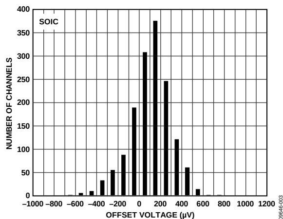
Figure 9. Input Offset Voltage Distribution, V_{SV} = \pm 5\text{ V}
