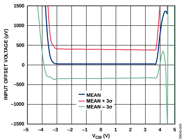
Figure 11. Input Offset Voltage vs. Common-Mode Input Voltage ( V_{CM} ), V_{SV} = \pm 5\text{ V} , R_L = \infty
