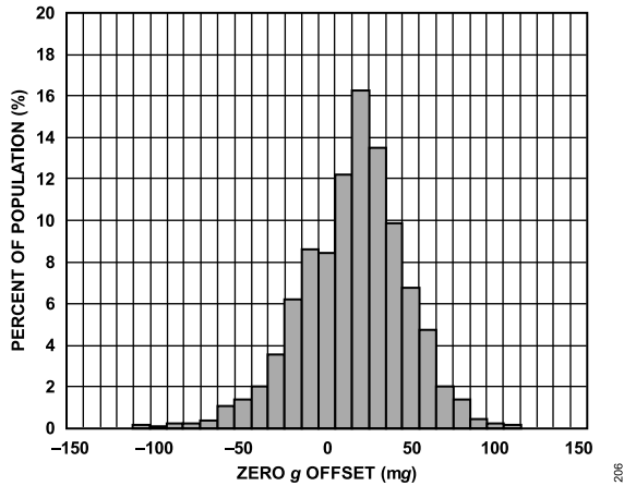
Figure 4. Zero g Offset at 25°C, V_S = 2.5\text{ V} , All Axes
