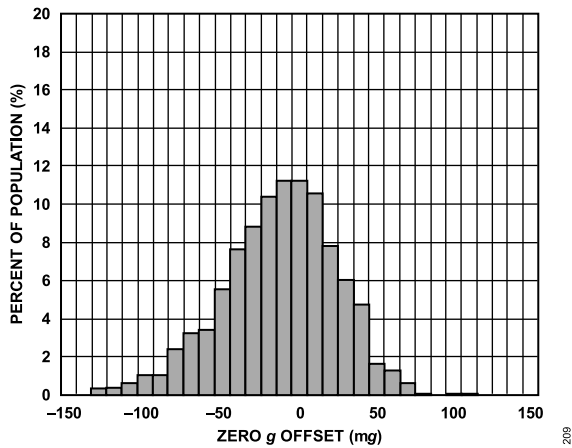
Figure 5. Zero g Offset at 25°C, V_S = 3.3\text{ V} , All Axes
