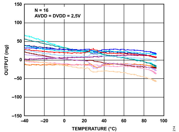
Figure 8. Y-Axis Zero g Offset vs. Temperature—Eight Parts Soldered to PCB, V_S = 2.5\text{ V}
