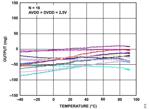
Figure 7. X-Axis Zero g Offset vs. Temperature—Eight Parts Soldered to PCB, V_S = 2.5\text{ V}
