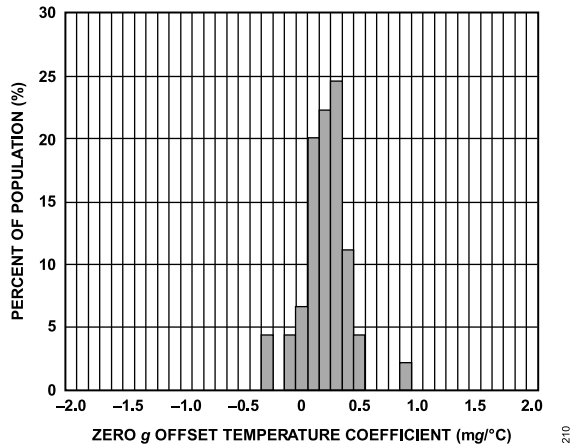
Figure 6. Zero g Offset Temperature Coefficient, V_S = 2.5\text{ V} , All Axes
