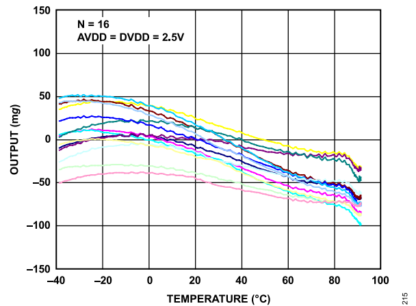
Figure 9. Z-Axis Zero g Offset vs. Temperature—Eight Parts Soldered to PCB, V_S = 2.5\text{ V}
