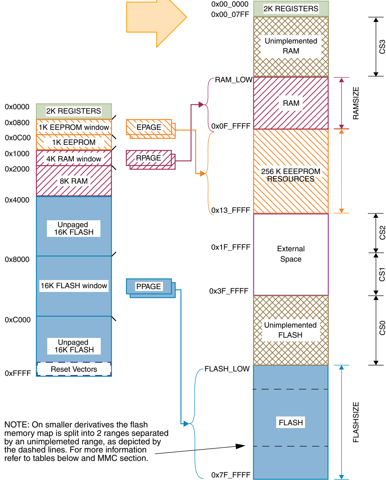
Figure 1-2. MC9S12XE100 Global Memory Map
