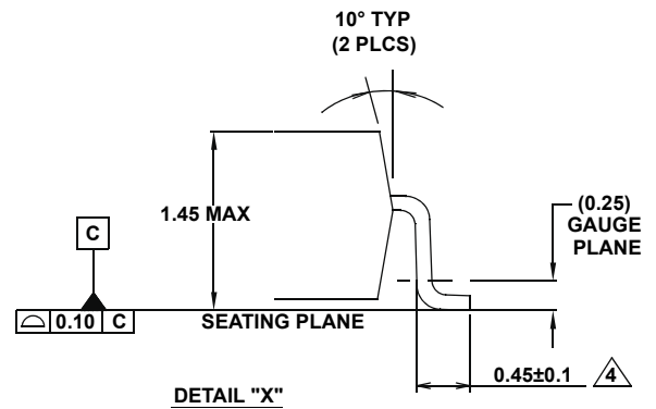
DETAIL "X"
