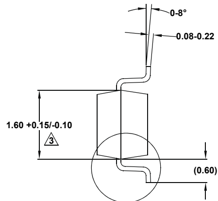
SEE DETAIL X END VIEW
