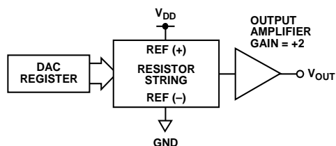
Figure 52. DAC Architecture
