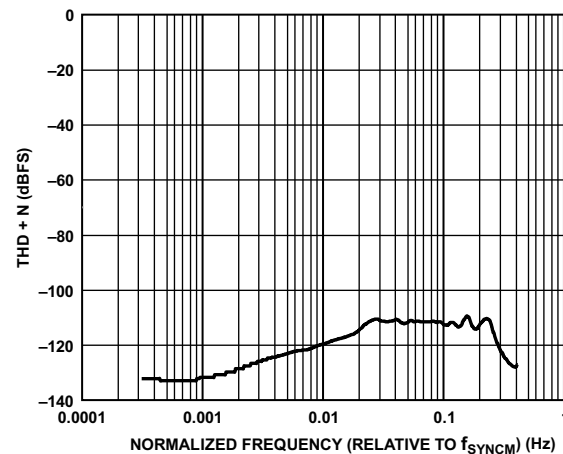
Figure 17. PDM Total Harmonic Distortion + Noise (THD + N) vs. Normalized Frequency (Relative to f_{\text{SYNC}} )
