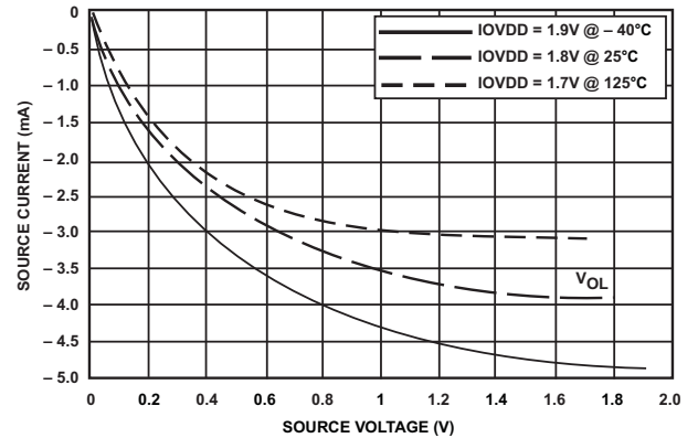
Figure 22. \bar{P} C Drivers (1.8 V IOVDD)
