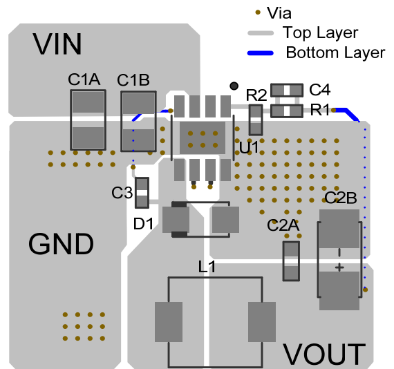
Figure 3: Recommended Layout
