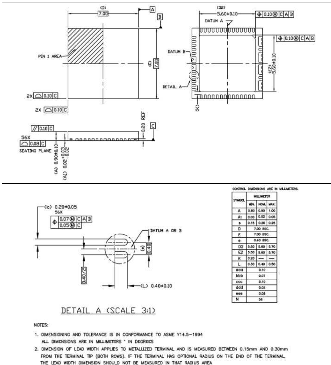
Figure 38 Package information
